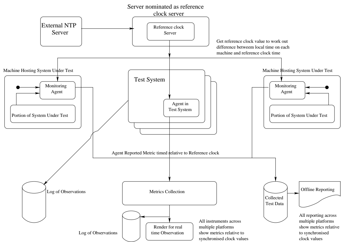
Figure 1: Overview of a System under Test using a Code Magus Limited Reference Clock implementation
